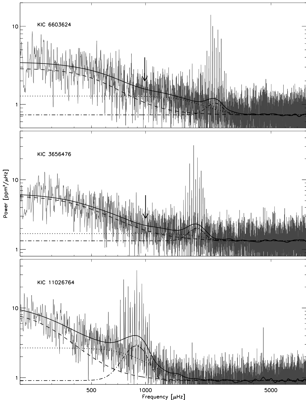
Fig. 1.— Frequency-power spectra of the three stars, smoothed over 1 \mu\text{Hz} , plotted on a log-log scale (grey). The continuous black lines show heavily smoothed spectra (Gaussian filter). The other lines show best-fitting estimates of different components: the power envelope due to oscillations, added to the offset from shot noise (dot-dashed); faculae (dotted) and active regions (dashed). The arrows indicate the location of the active region (see text).
