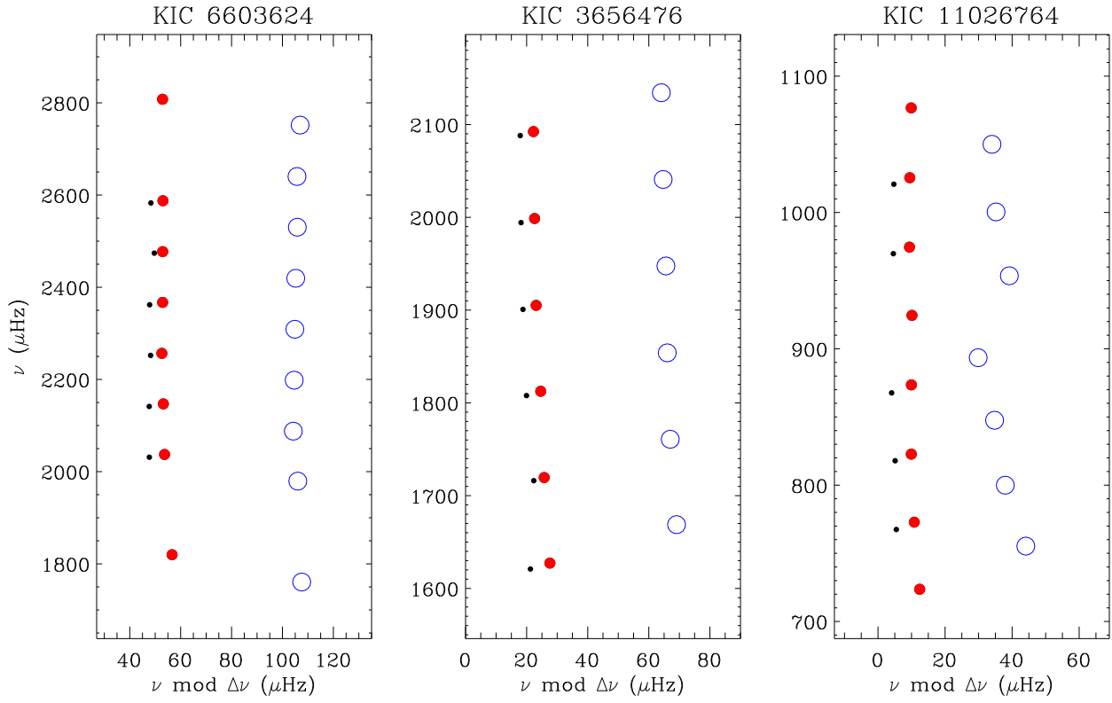
Fig. 3.— Échelle diagrams of the observed frequencies in each star, showing the l = 0 (filled red symbols), l = 1 (open blue symbols) and l = 2 (small black symbols) ridges.
