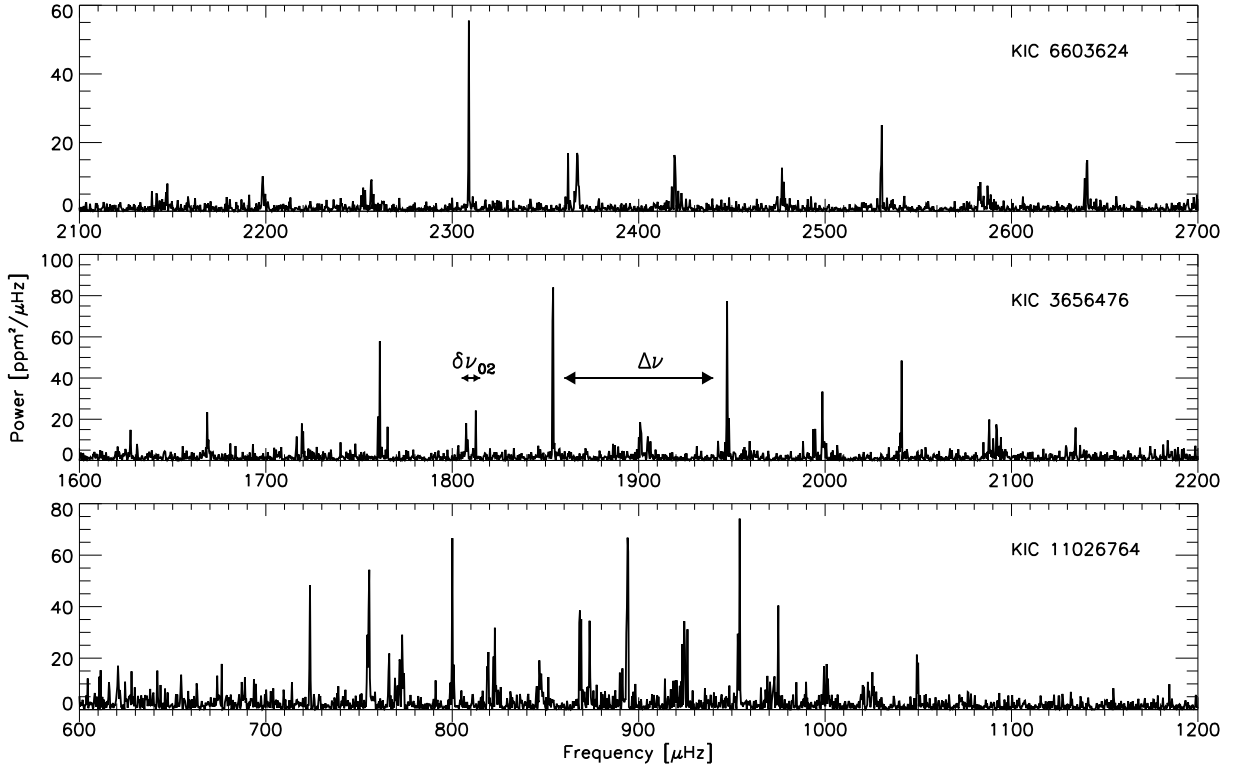
Fig. 2.— Frequency-power spectra of the three stars, plotted on a linear scale over the frequency ranges where the mode amplitudes are most prominent. Examples of the characteristic large ( \Delta\nu ) and small ( \delta\nu_{02} ) frequency separations are also marked on the spectrum of KIC 3656476.
