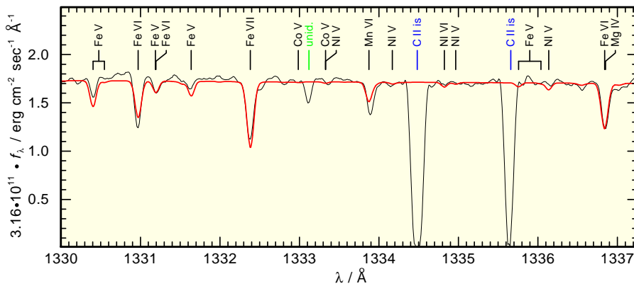
Fig. 3. Modelling the ionization equilibrium of Fe V – Fe VII. It is well matched at T_{\text{eff}} = 95 kK. Ionization equilibria are sensitive indicators for T_{\text{eff}} . The marks indicate the positions of identified lines (is denotes interstellar lines, unid. is an unidentified line).
