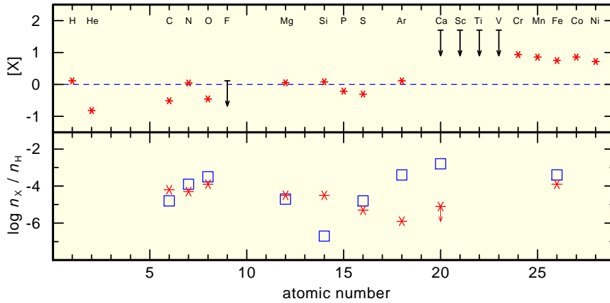
Fig. 4. Top: Photospheric element abundances of LS V +46°21 determined from detailed line profile fits. [x] denotes \log (mass fraction / solar mass fraction) of species x . The dashed, horizontal line indicates the solar abundance values (Asplund, Grevesse & Sauval 2005). For F, Ca, Sc, Ti, and V upper limits can be found only. Bottom: Comparison of the elemental number ratios found in our spectral analysis (red stars) compared to predictions (blue squares) of diffusion calculations for DA models (Chayer et al. 1995) with T_{\text{eff}} = 95 kK and \log g = 7 .
