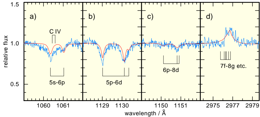
Fig. 2. Identification of Ne VIII lines in the FUSE (panels a – c) and HST/GHRS (panel d) observations of the extremely hot ( T_{\text{eff}} = 170 \text{ kK} ) CS of MWP 1 (PNG080.3–10.4, Motch, Werner & Pakull 1993), RX J2117.1+3412 (Werner et al. 2007). Note that the C IV doublet in panel a is not included in the model.
