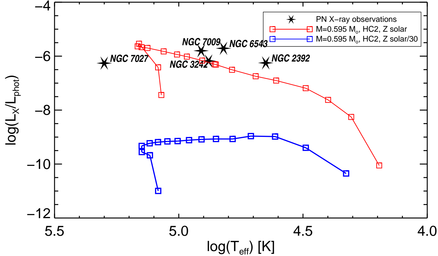
X-ray Luminosity ( 5 – 28 Å) over Photon Luminosity
