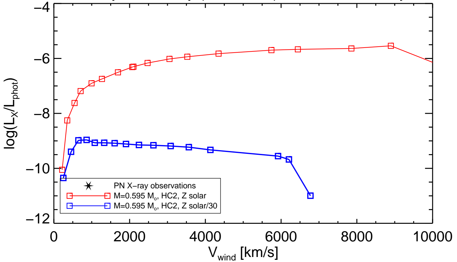
X-ray Luminosity ( 5 – 28 Å) over Wind Velocity
