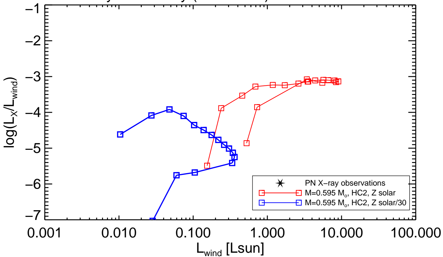
X-ray Luminosity ( 5 – 28 Å) over Wind Power
