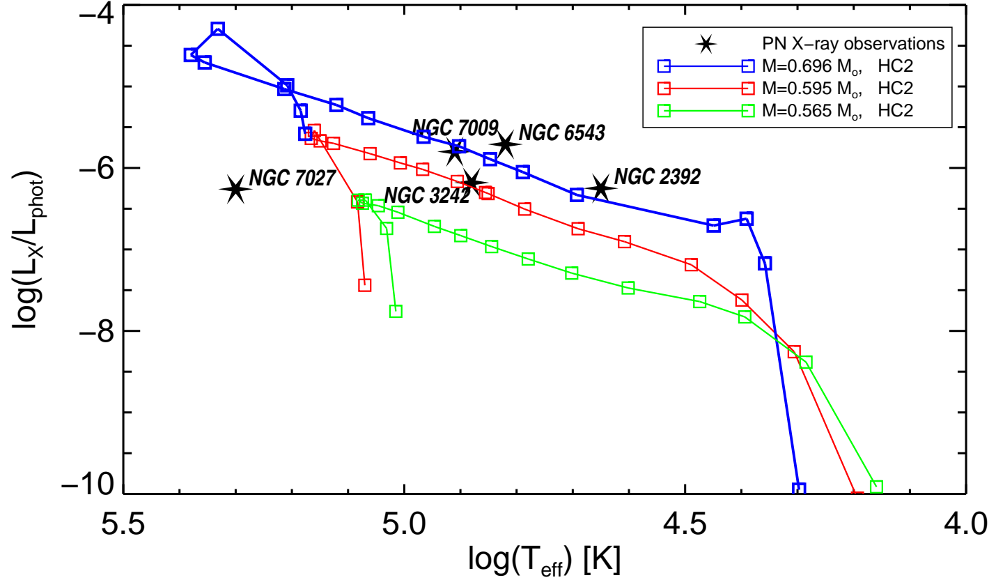
X-ray Luminosity ( 5 – 28 Å) over Photon Luminosity
