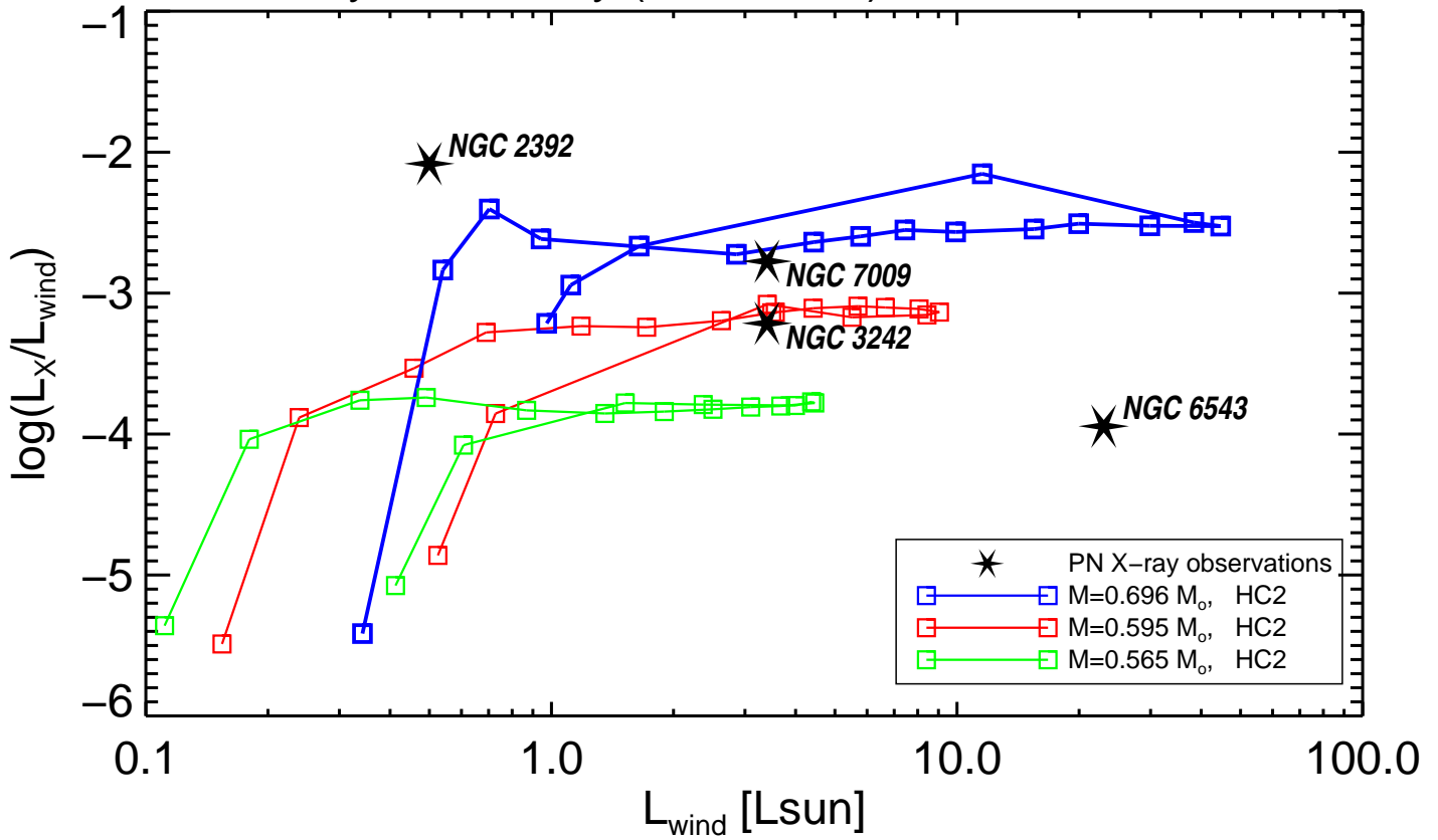
X-ray Luminosity ( 5 – 28 Å) over Wind Power
