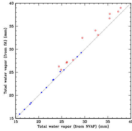
Figure 3. Comparison of direct and integrated water vapor column data. Fill blue circles correspond to La Palma and red open circles to Mauna Kea.
