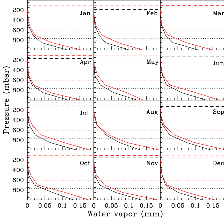
Figure 2. Water vapor function at Mauna Kea (red) and La Palma (black). Dotted horizontal lines correspond to observatories altitudes (mean pressure level at the observatories). Dashed lines corresponds to the monthly average pressure at the tropopause level.
