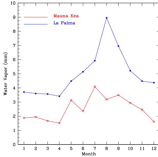
Figure 4. Monthly water vapor column (mm) in Mauna Kea (red) and La PALma (blue). We have integrated the water vapor function from the observatory level to the tropopause level.
